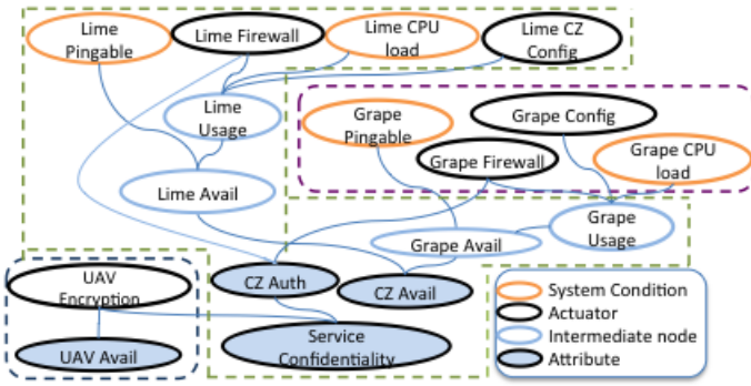
Figure 1: Cause-effect network distributed across lime , grape and UAV
